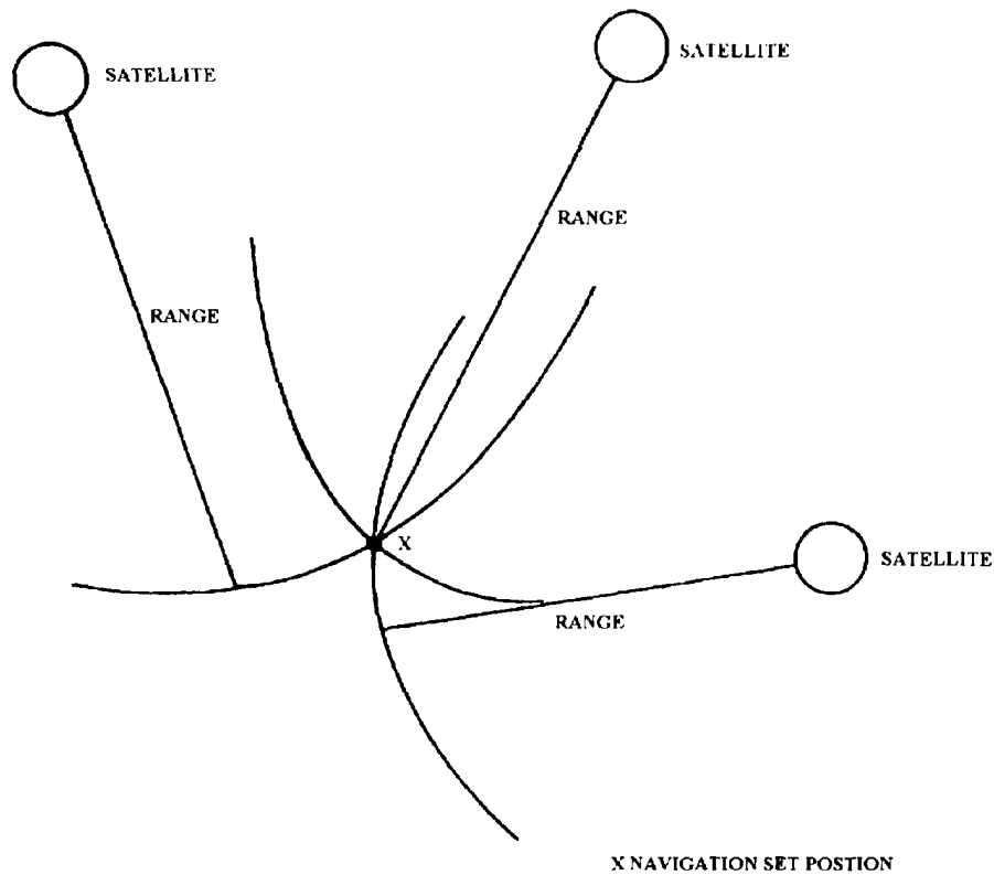
Figure 1-12.—Satellite ranging.
