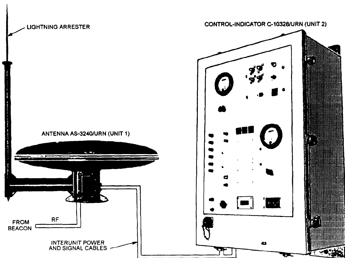
Figure 2-8.—Antenna Group OE-273(V)/URN.
