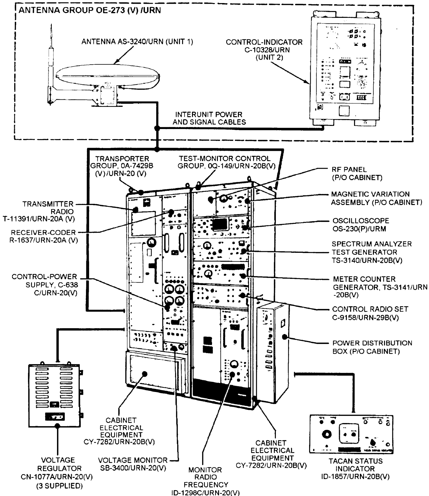
Figure 2-9.—TACAN Set AN/URN-20(V)1.
