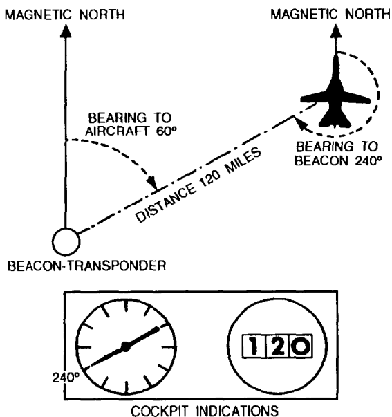
Figure 2-1.—TACAN aircraft indication.
