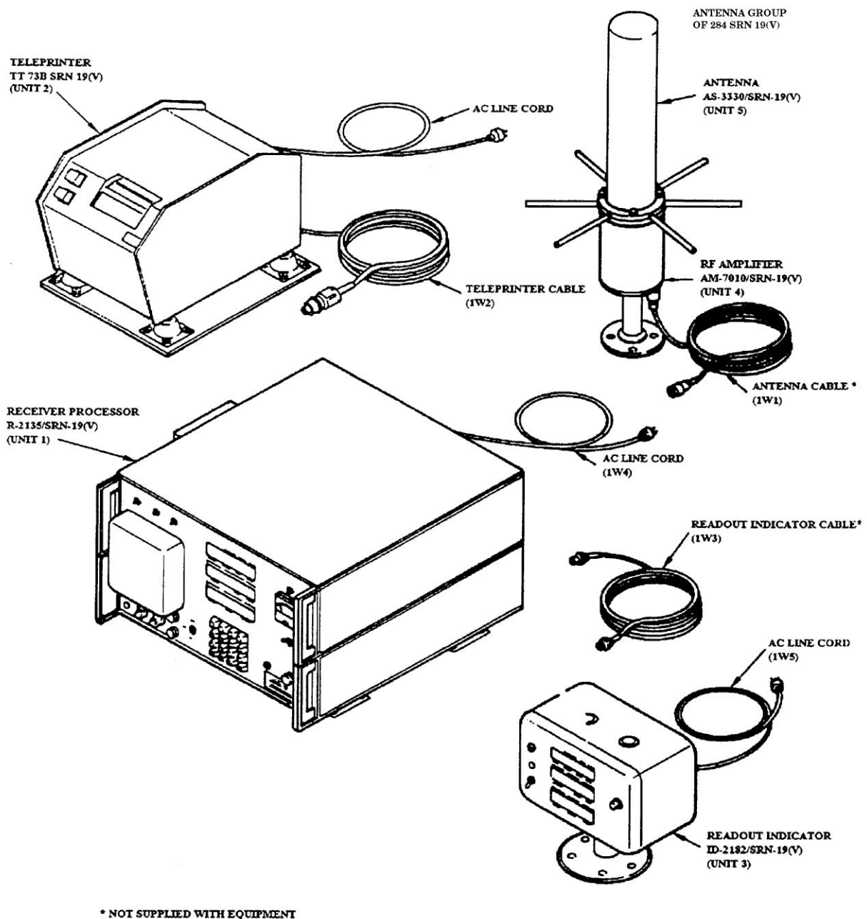
Figure 1-9.—AN/SRN-19(V)2 major components.
