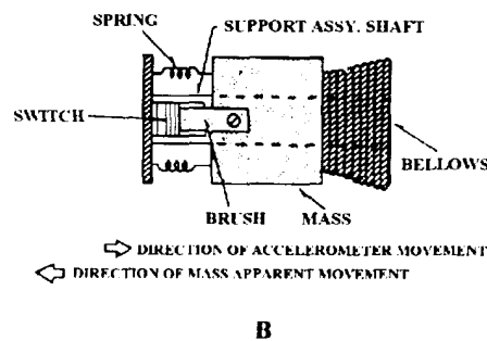
Figure 1-3.—Pulse counting accelerometer.
