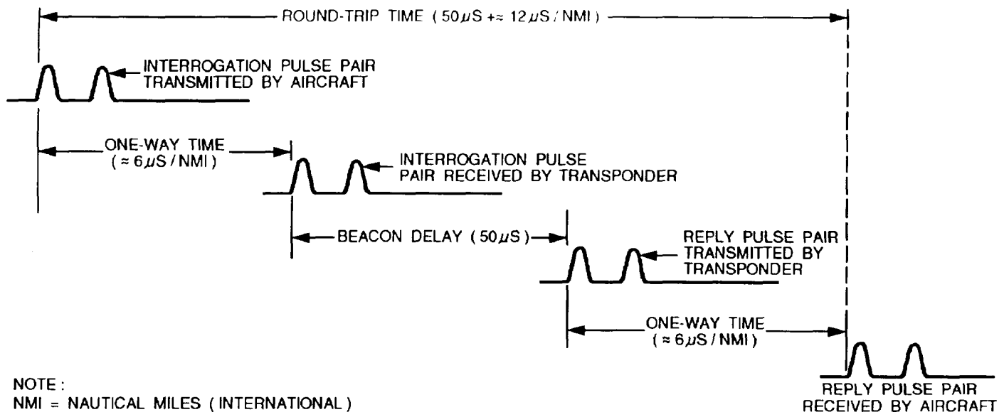
Figure 2-2.—Distance measuring round-trip travel time.
