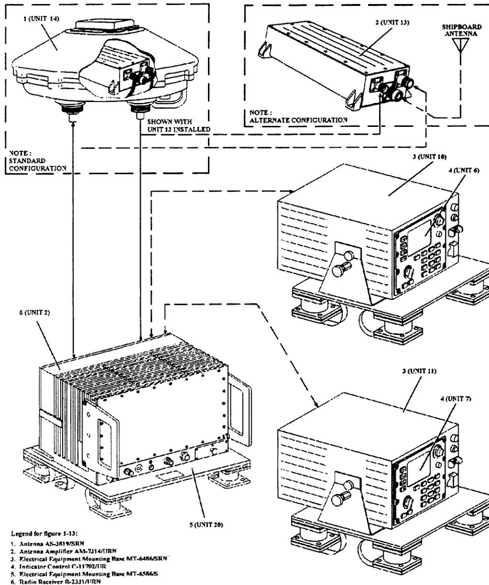
Figure 1-13.—Satellite Navigation Set AN/WRN-6(V).
