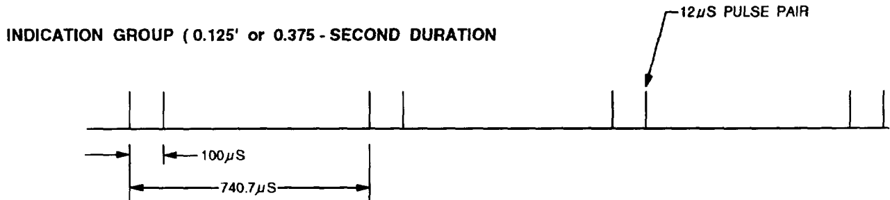
Figure 2-4.—Transponder output pulse train.
