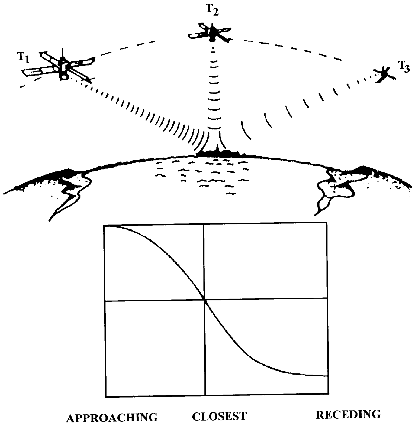
Figure 1-7.—Doppler shift relative to satellite transmitted frequency.
