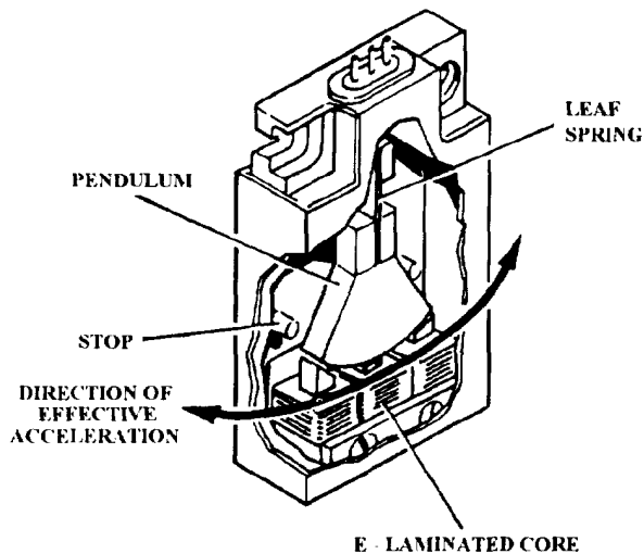
Figure 1-2.—E-transformer accelerometer.
