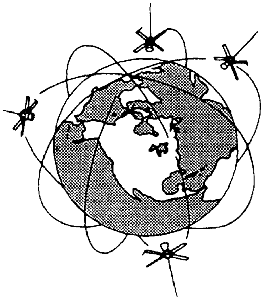
Figure 1-6.—Satellite orbits.
