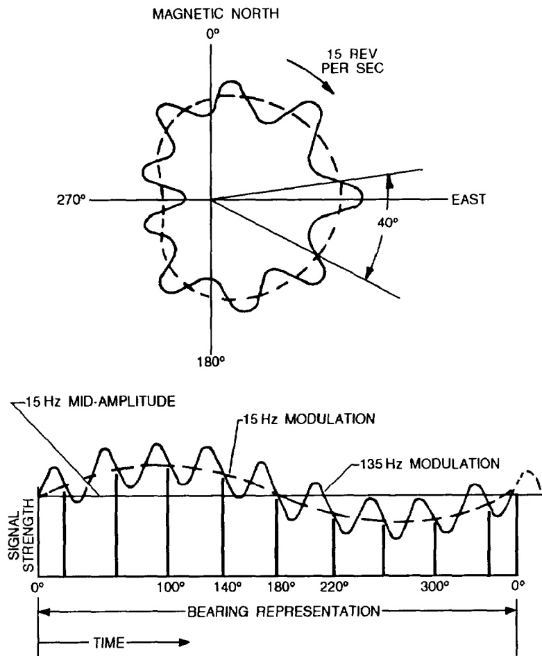
Figure 2-6.—TACAN modulation envelope
