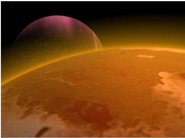
Proxima Centauri
